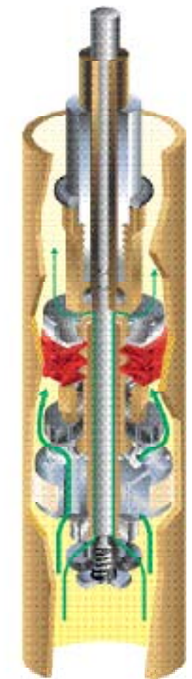
LARGE HIT Low-speed port open Shim stack open Spike valve open
